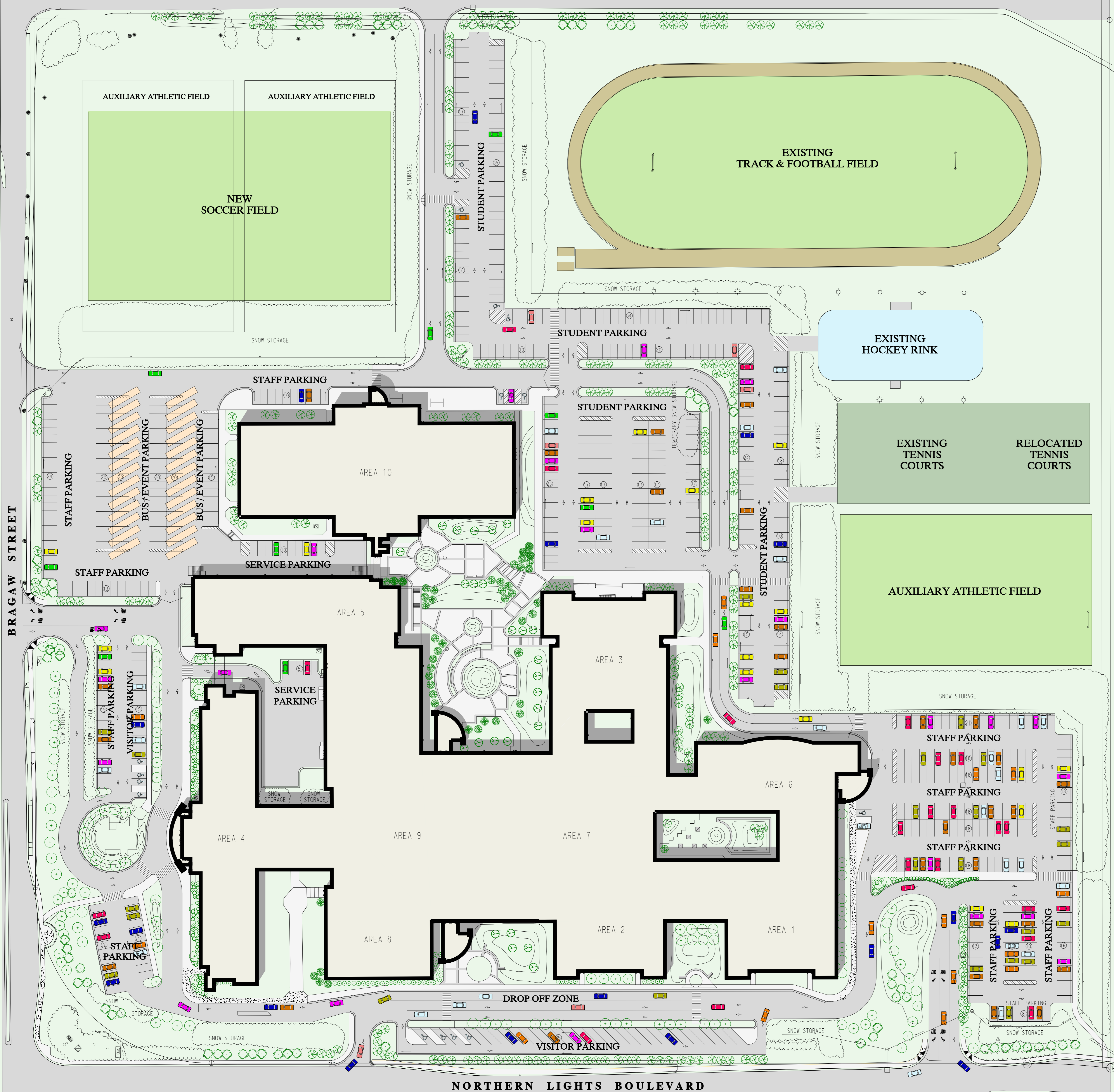
1 Master Site Plan Scale: 1" = 50' 0 10' 25' 50' 100'
